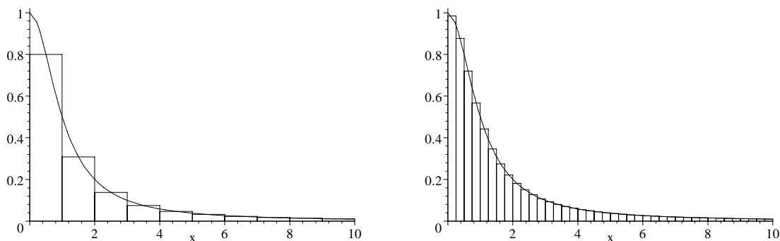
Fig. 1. Interpolation of the integral \int_0^{10} \frac{1}{x^2+1} dx with 10 and 40 intervals.
